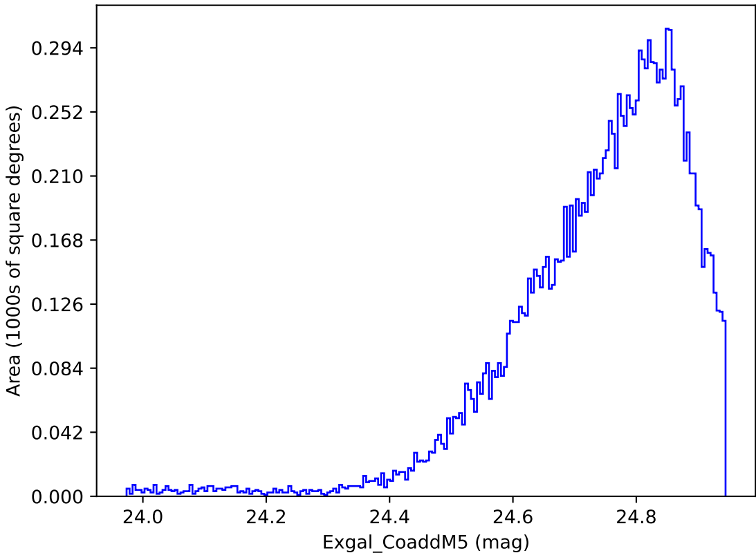
too_elab_r32_d3_griz_v3.4_10yrs WFD y band: Exgal_CoaddM5
