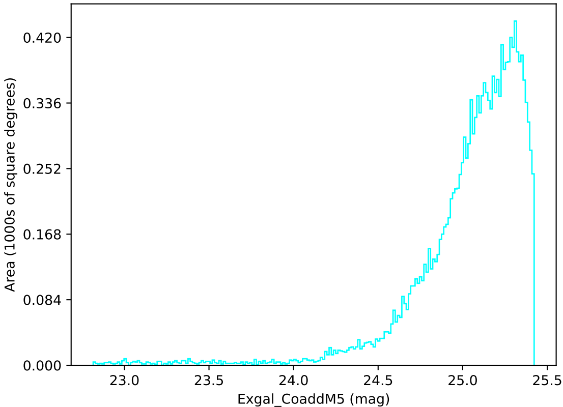
too_elab_r32_d3_griz_v3.4_10yrs WFD u band: Exgal_CoaddM5
