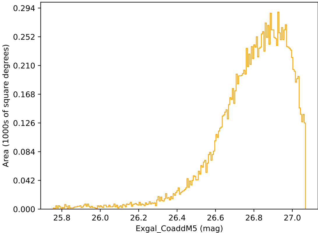
too_elab_r32_d3_griz_v3.4_10yrs WFD r band: Exgal_CoaddM5
