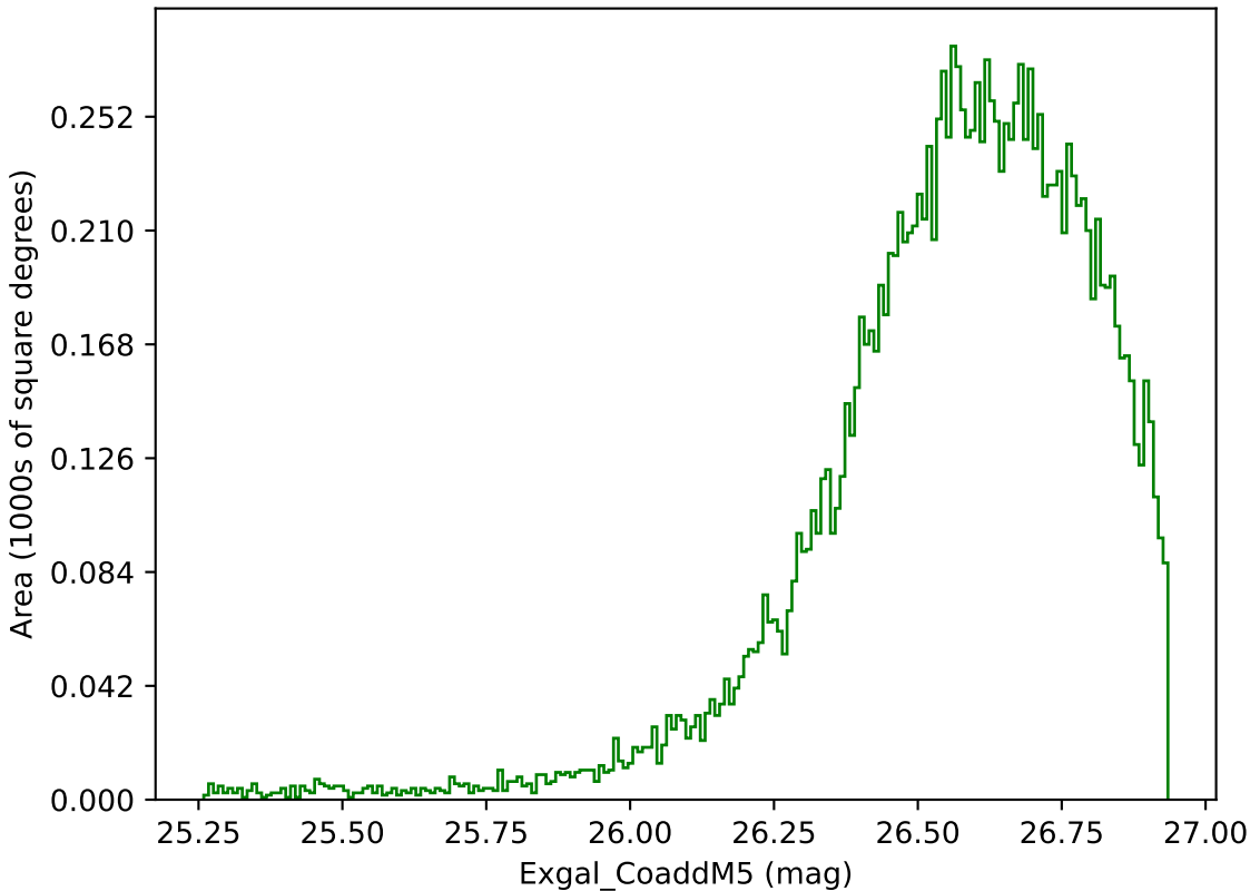
too_elab_r32_d3_griz_v3.4_10yrs WFD g band: Exgal_CoaddM5
