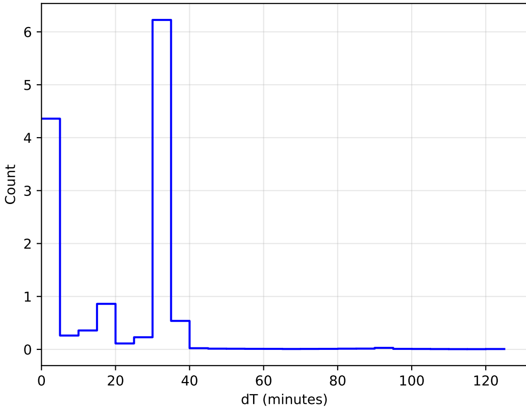
too_elab_r32_d3_griz_v3.4_10yrs All sky: DeltaT Histogram 1e6
