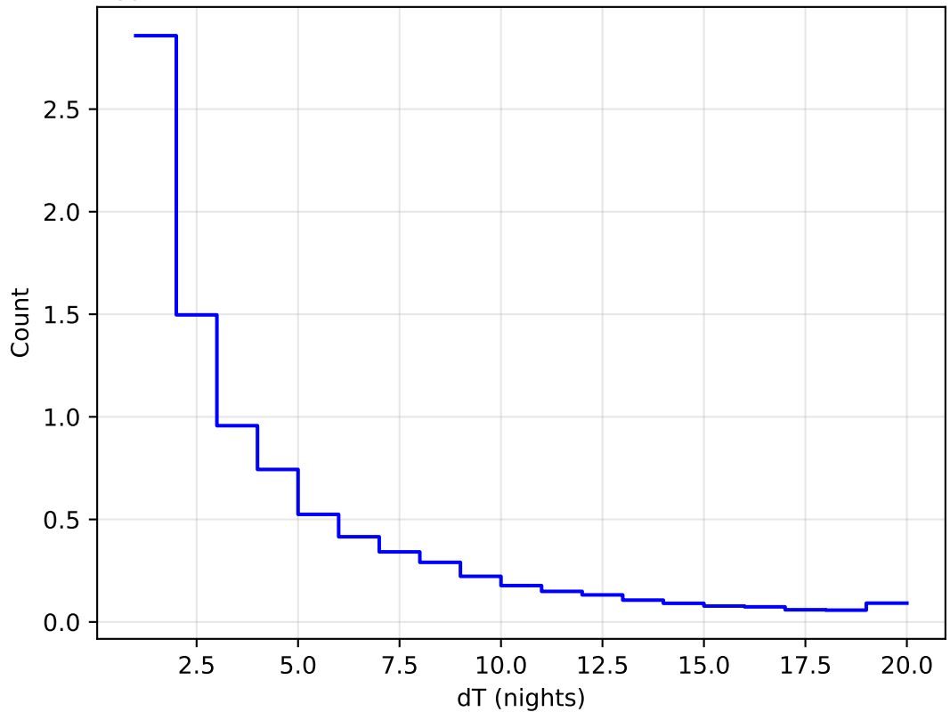
too_elab_r32_d3_griz_v3.4_10yrs All sky all bands: DeltaNight Histogram
