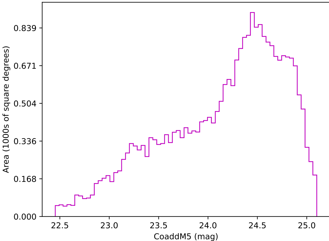
too_elab_r32_d3_griz_v3.4_10yrs Yr 3-4 z band: CoaddM5
