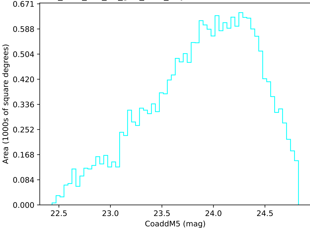
too_elab_r32_d3_griz_v3.4_10yrs Yr 3-4 u band: CoaddM5
