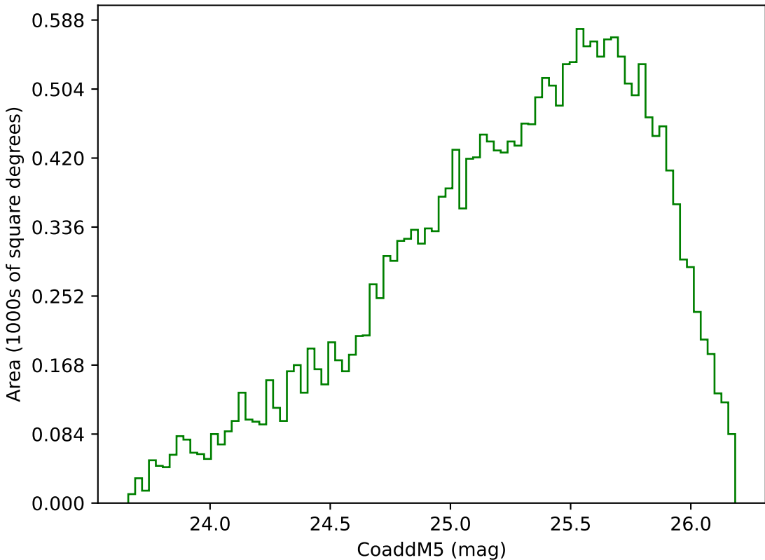
too_elab_r32_d3_griz_v3.4_10yrs Yr 3-4 g band: CoaddM5
