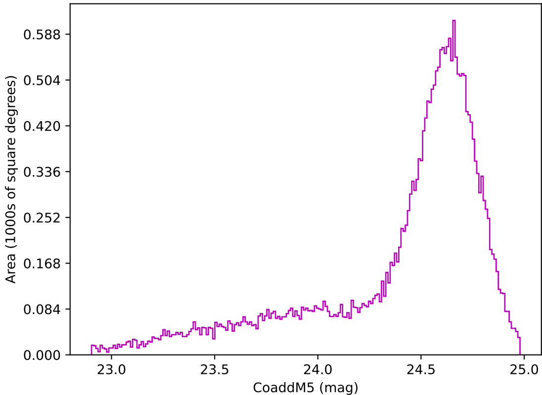
too_elab_r32_d3_griz_v3.4_10yrs Yr 1 z band: CoaddM5
