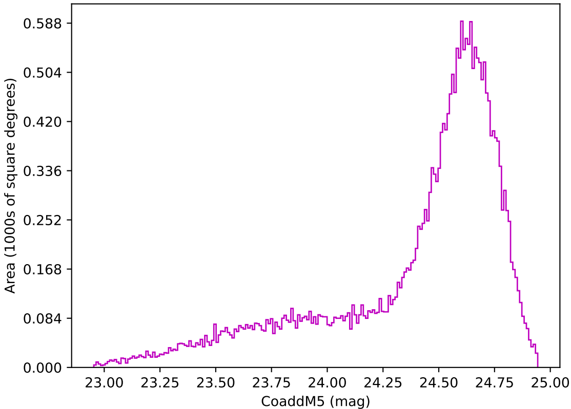
too_elab_r32_d3_griz_v3.4_10yrs Yr 1 z band: CoaddM5
