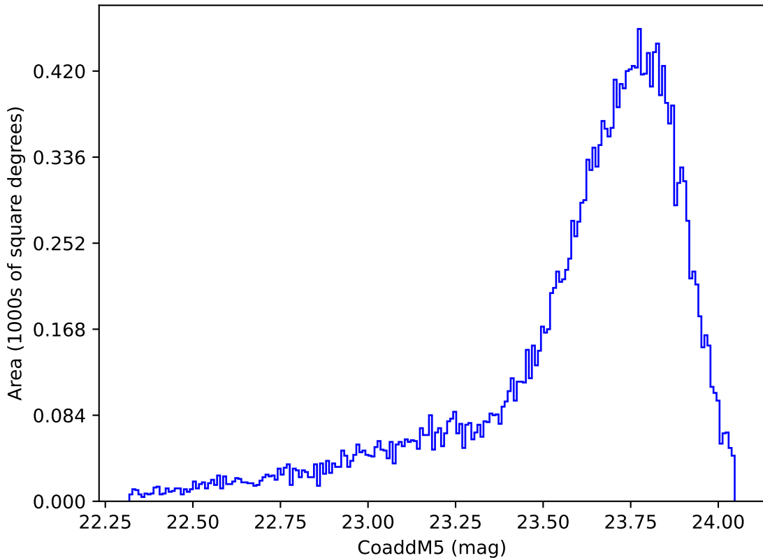
too_elab_r32_d3_griz_v3.4_10yrs Yr 1 y band: CoaddM5
