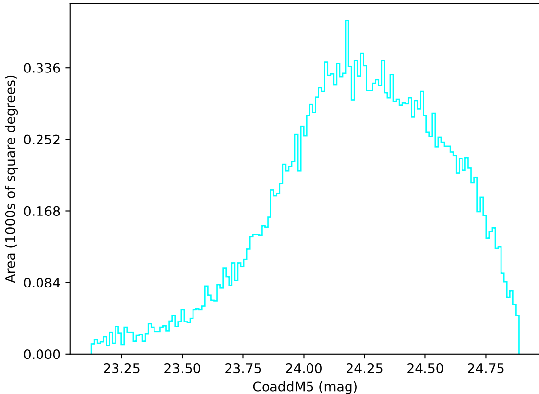
too_elab_r32_d3_griz_v3.4_10yrs Yr 1 u band: CoaddM5
