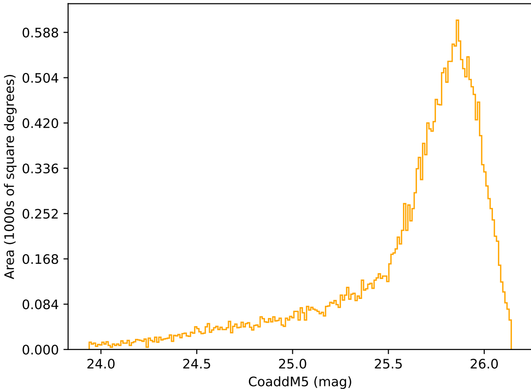
too_elab_r32_d3_griz_v3.4_10yrs Yr 1 r band: CoaddM5
