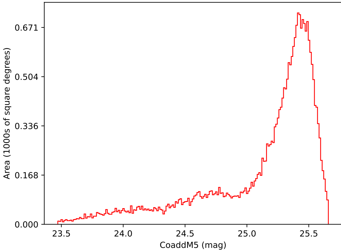
too_elab_r32_d3_griz_v3.4_10yrs Yr 1 i band: CoaddM5
