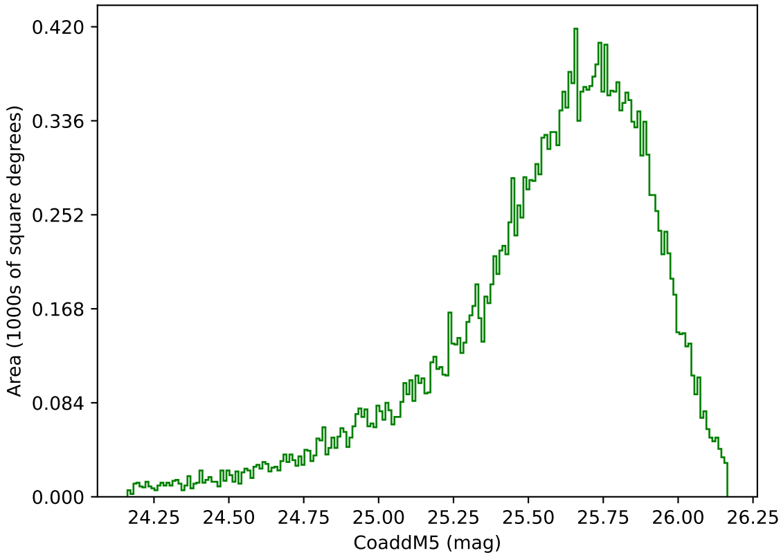
too_elab_r32_d3_griz_v3.4_10yrs Yr 1 g band: CoaddM5
