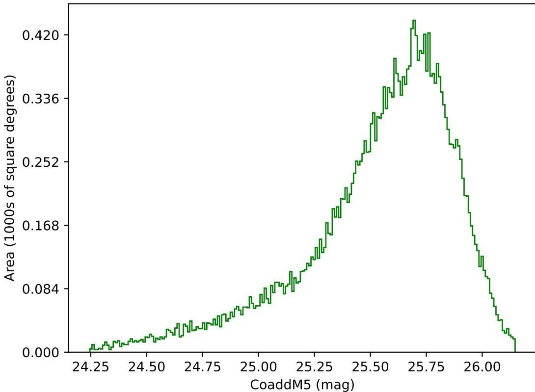
too_elab_r32_d3_griz_v3.4_10yrs Yr 1 g band: CoaddM5
