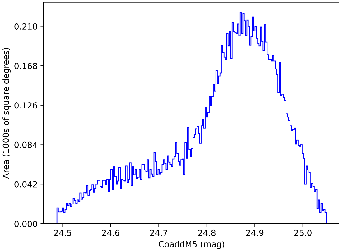
too_elab_r32_d3_griz_v3.4_10yrs WFD y band: CoaddM5
