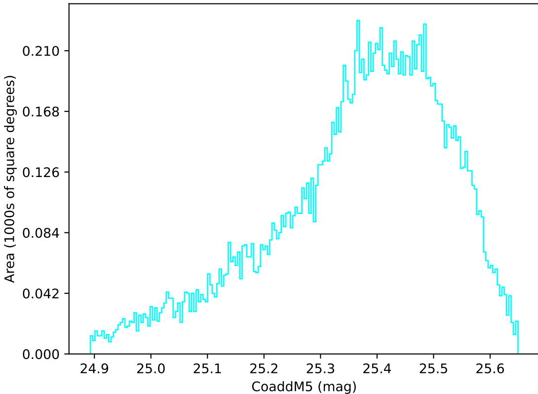
too_elab_r32_d3_griz_v3.4_10yrs WFD u band: CoaddM5
