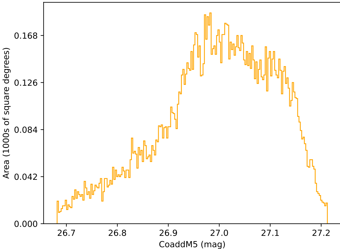
too_elab_r32_d3_griz_v3.4_10yrs WFD r band: CoaddM5
