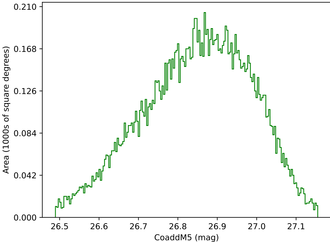
too_elab_r32_d3_griz_v3.4_10yrs WFD g band: CoaddM5
