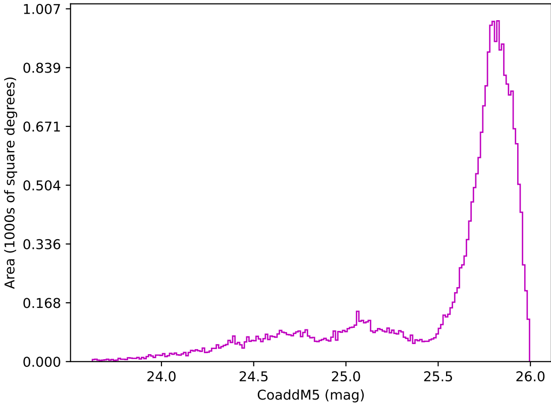
too_elab_r32_d3_griz_v3.4_10yrs All sky z band: CoaddM5
