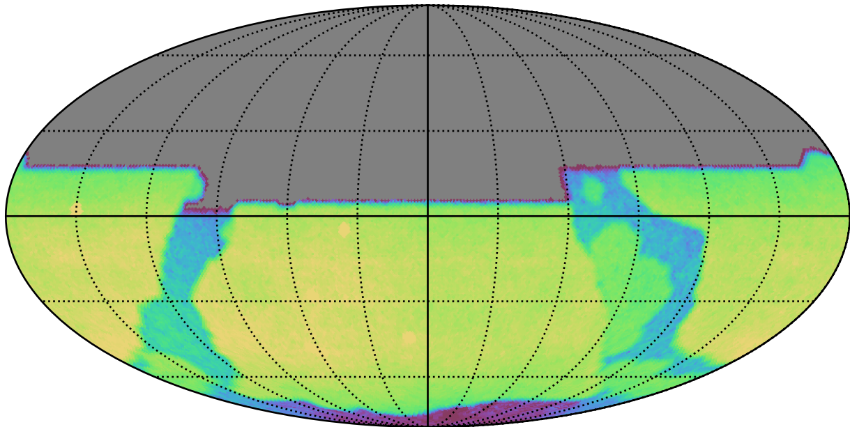
too_elab_r32_d3_griz_v3.4_10yrs All sky y band: CoaddM5
