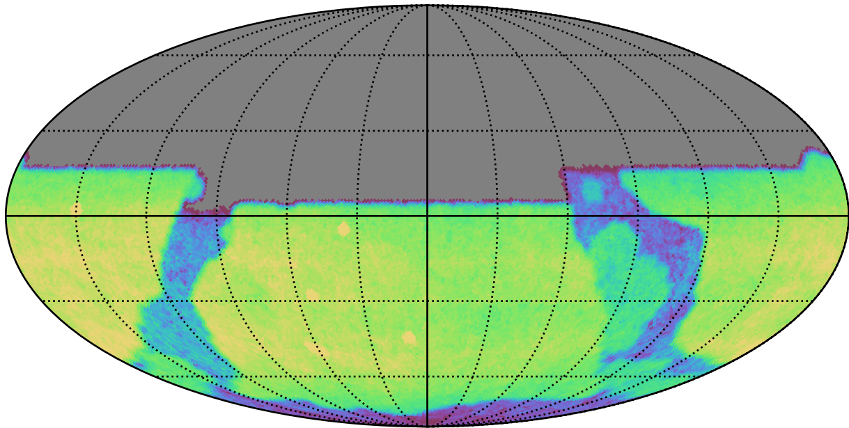
too_elab_r32_d3_griz_v3.4_10yrs All sky u band: CoaddM5
