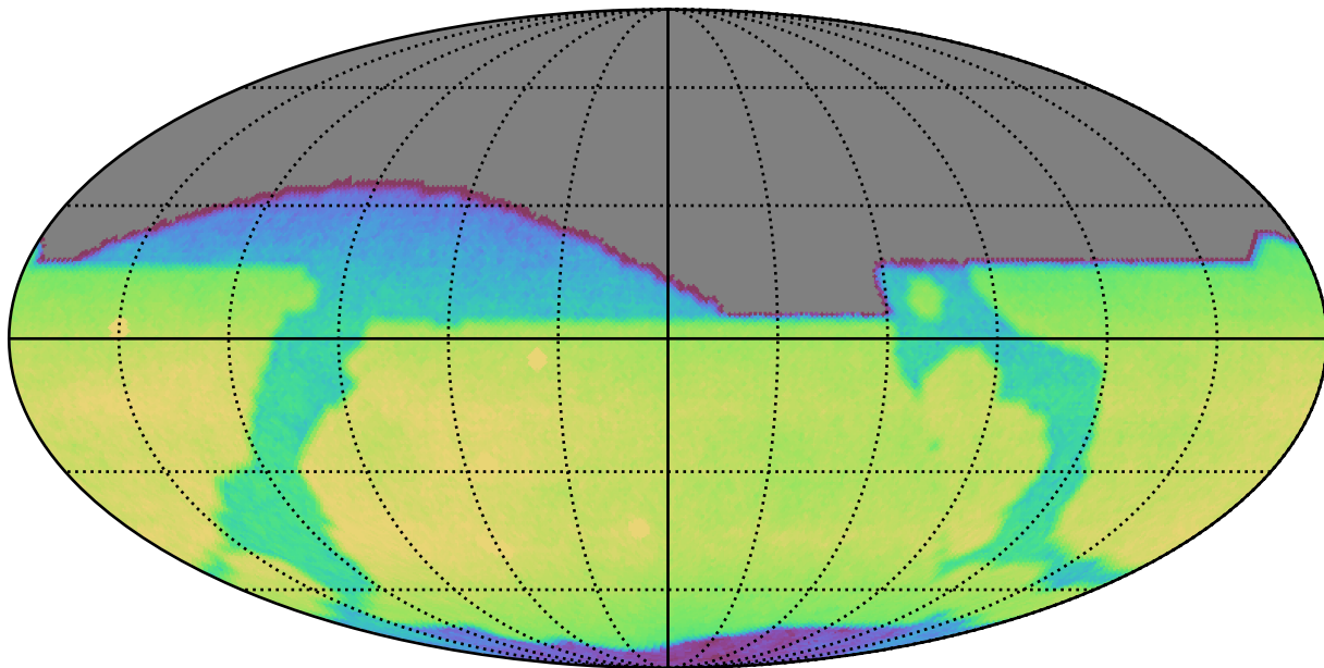
too_elab_r32_d3_griz_v3.4_10yrs All sky i band: CoaddM5
