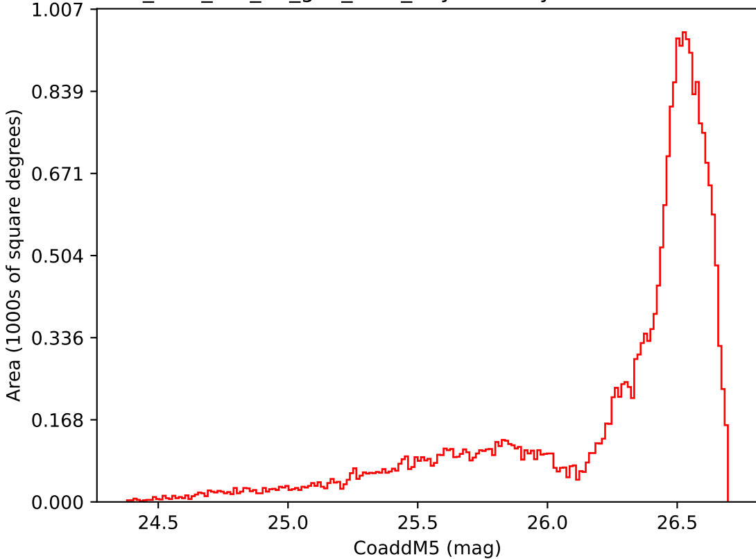
too_elab_r32_d3_griz_v3.4_10yrs All sky i band: CoaddM5
