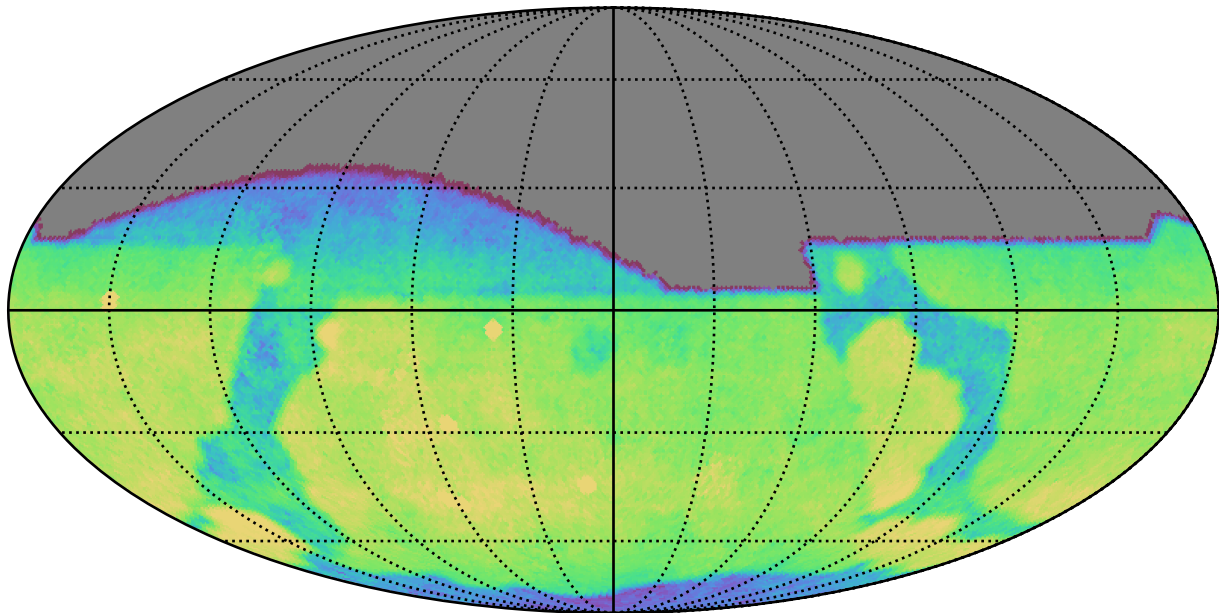
too_elab_r32_d3_griz_v3.4_10yrs All sky g band: CoaddM5
