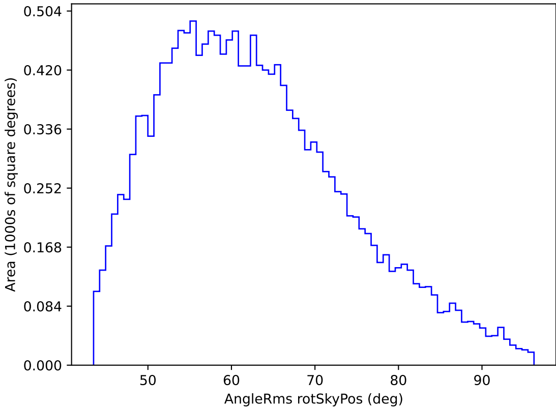
too_elab_r32_d3_griz_v3.4_10yrs WFD u band: AngleRms rotSkyPos
