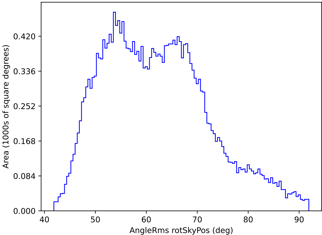
too_elab_r32_d3_griz_v3.4_10yrs All sky i band: AngleRms rotSkyPos
