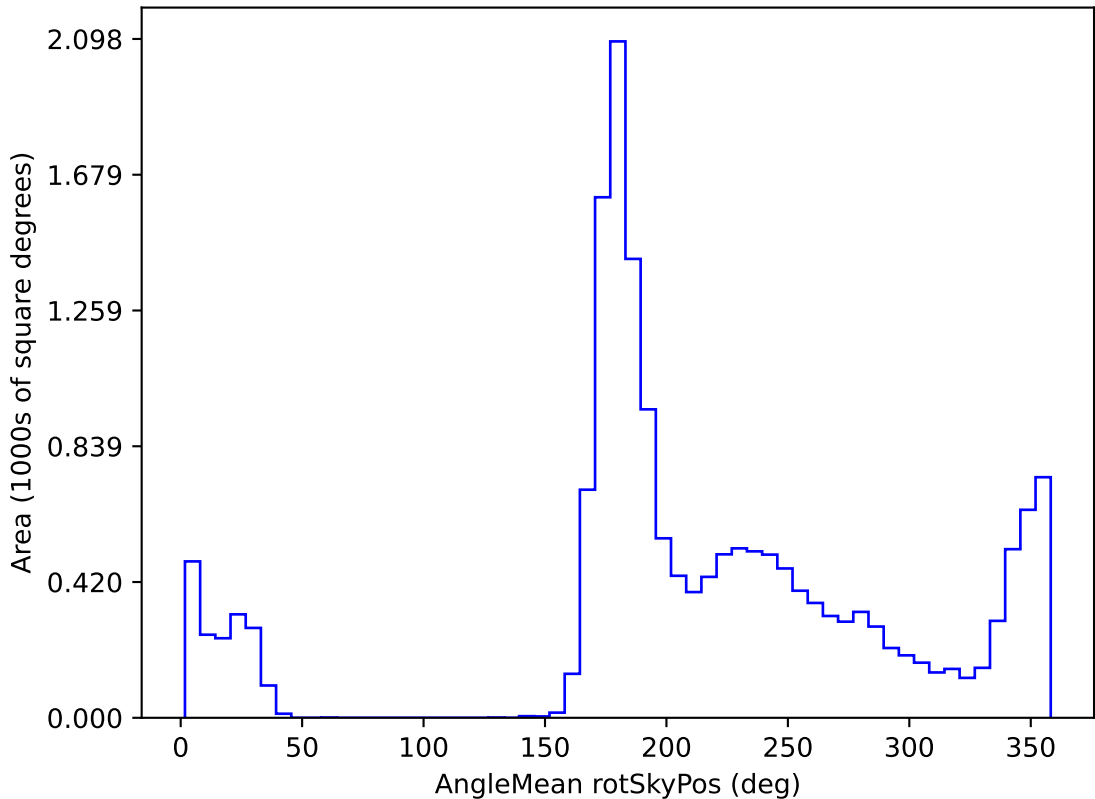
too_elab_r32_d3_griz_v3.4_10yrs WFD r band: AngleMean rotSkyPos
