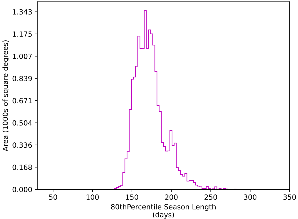
too_elab_r32_d3_griz_v3.4_10yrs WFD z band: 80thPercentile Season Length
