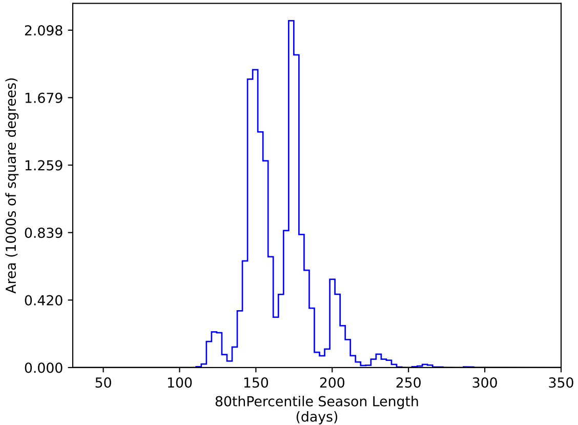
too_elab_r32_d3_griz_v3.4_10yrs WFD y band: 80thPercentile Season Length
