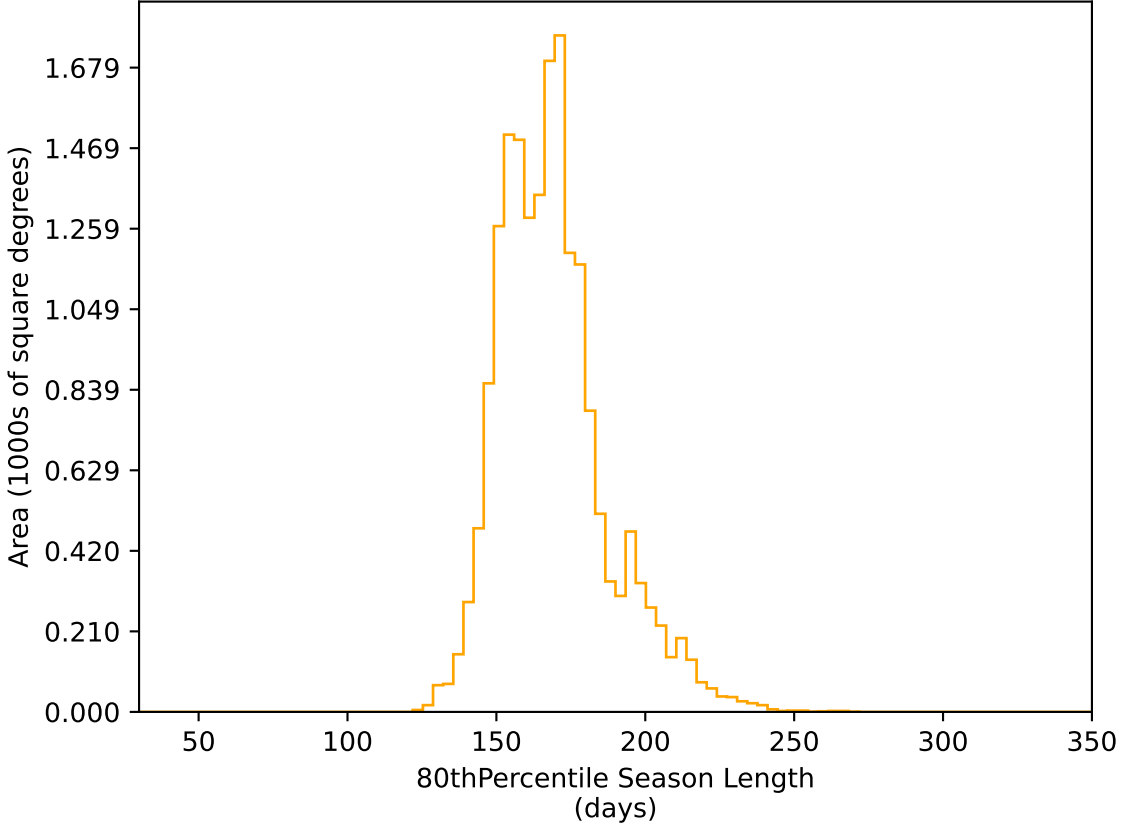
too_elab_r32_d3_griz_v3.4_10yrs WFD r band: 80thPercentile Season Length
