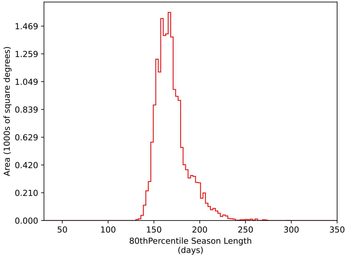
too_elab_r32_d3_griz_v3.4_10yrs WFD i band: 80thPercentile Season Length
