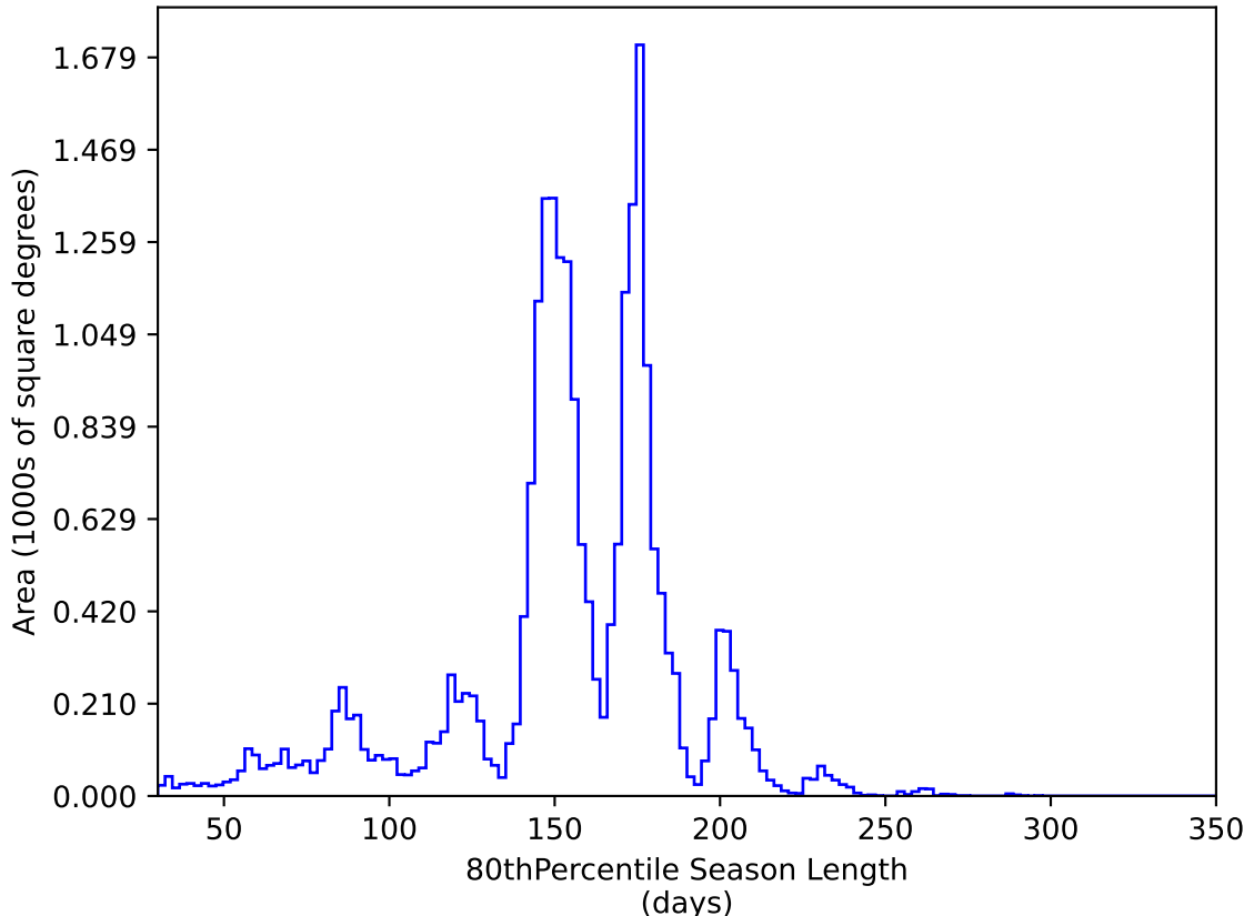
too_elab_r32_d3_griz_v3.4_10yrs All sky y band: 80thPercentile Season Length
