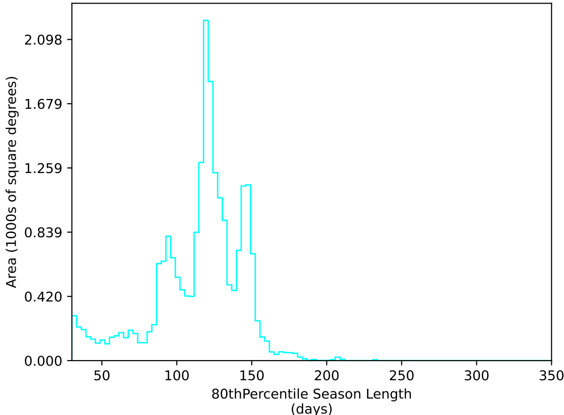
too_elab_r32_d3_griz_v3.4_10yrs All sky u band: 80thPercentile Season Length
