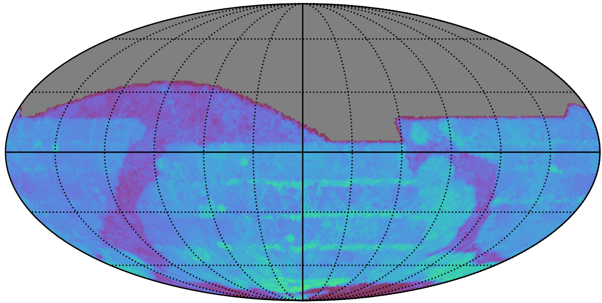
too_elab_r32_d3_griz_v3.4_10yrs All sky r band: 80thPercentile Season Length
