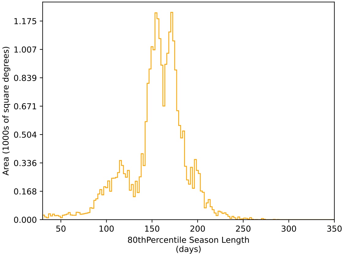
too_elab_r32_d3_griz_v3.4_10yrs All sky r band: 80thPercentile Season Length
