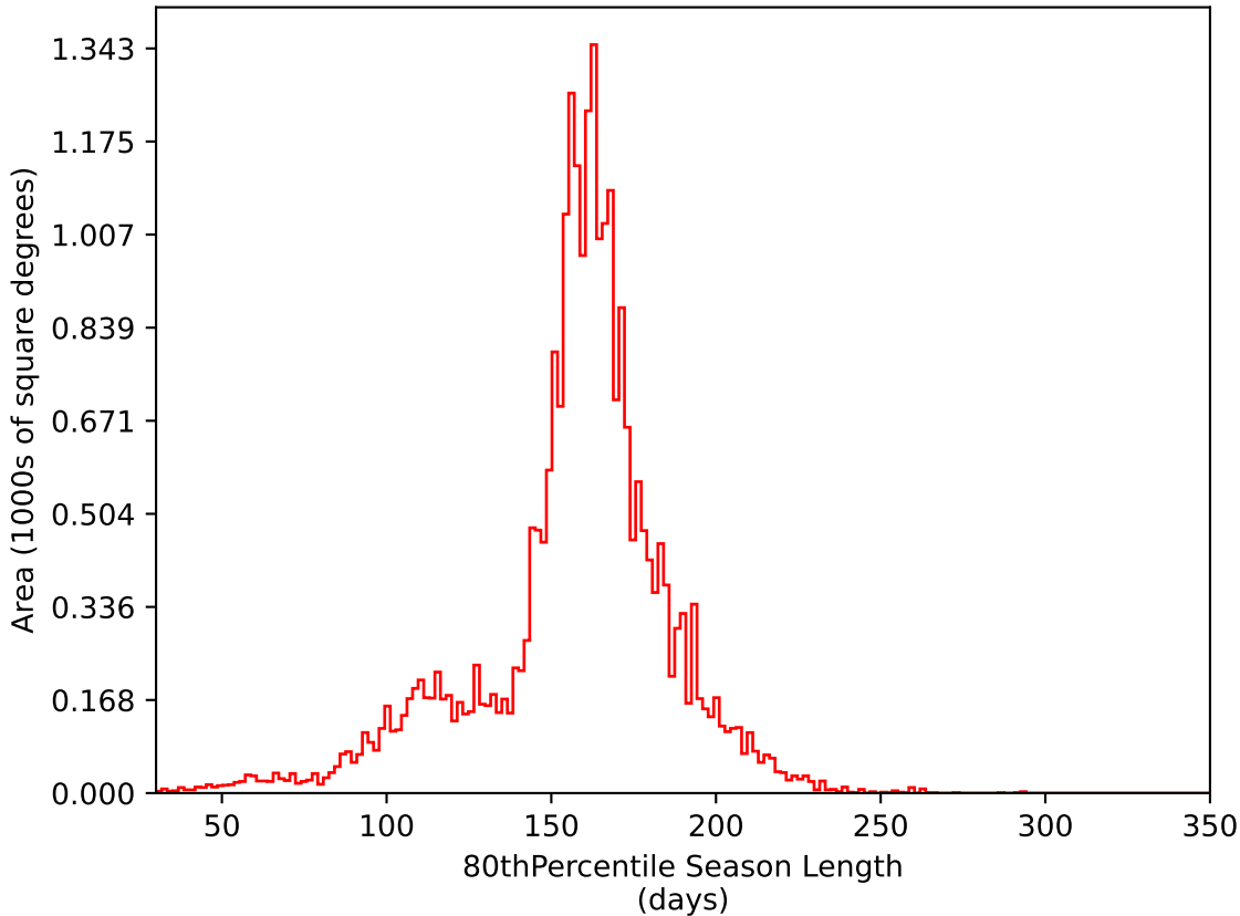
too_elab_r32_d3_griz_v3.4_10yrs All sky i band: 80thPercentile Season Length
