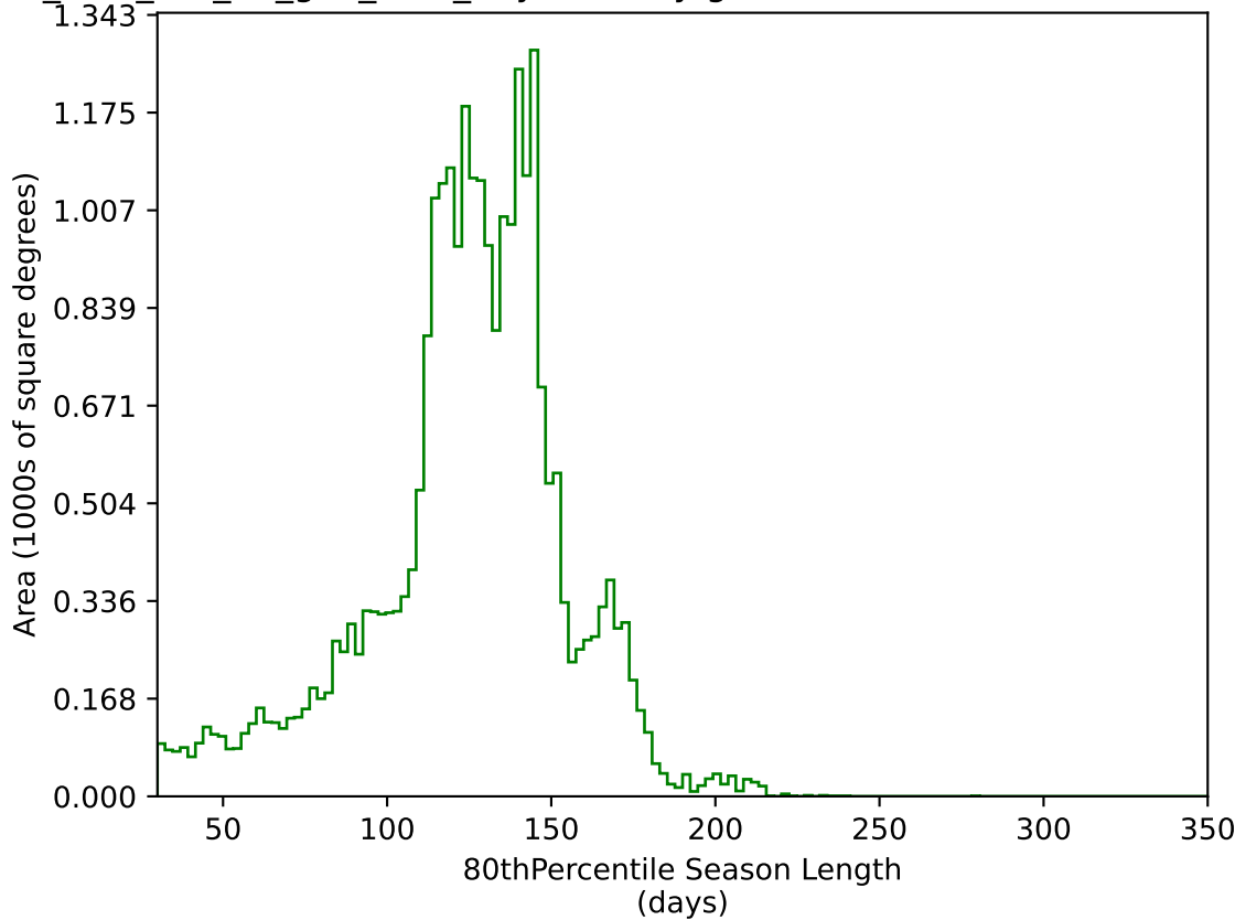
too_elab_r32_d3_griz_v3.4_10yrs All sky g band: 80thPercentile Season Length
