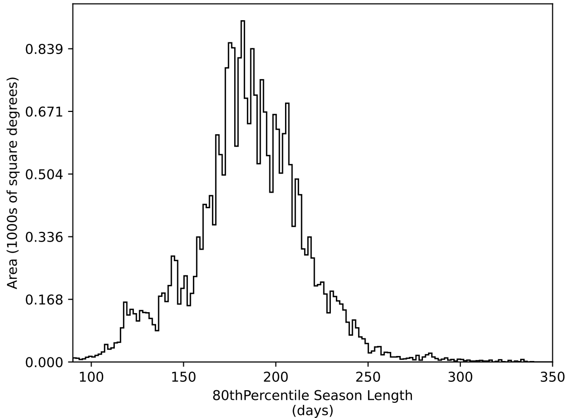
too_elab_r32_d3_griz_v3.4_10yrs All sky all bands: 80thPercentile Season Length
