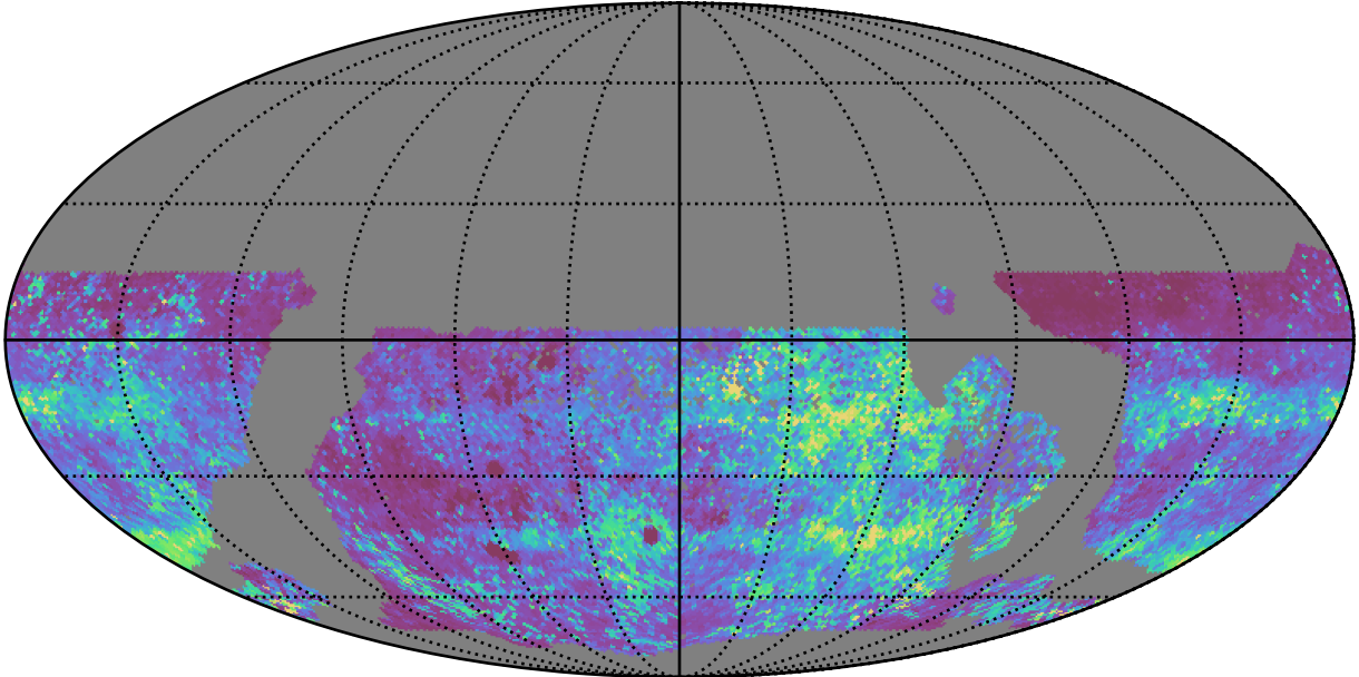
too_elab_r32_d3_griz_v3.4_10yrs WFD zy bands: 75th Percentile Intranight Timespan
