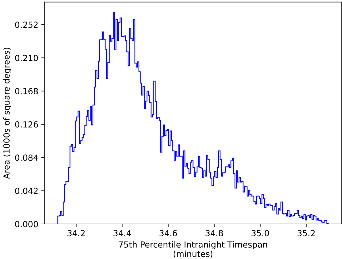
too_elab_r32_d3_griz_v3.4_10yrs WFD zy bands: 75th Percentile Intranight Timespan
