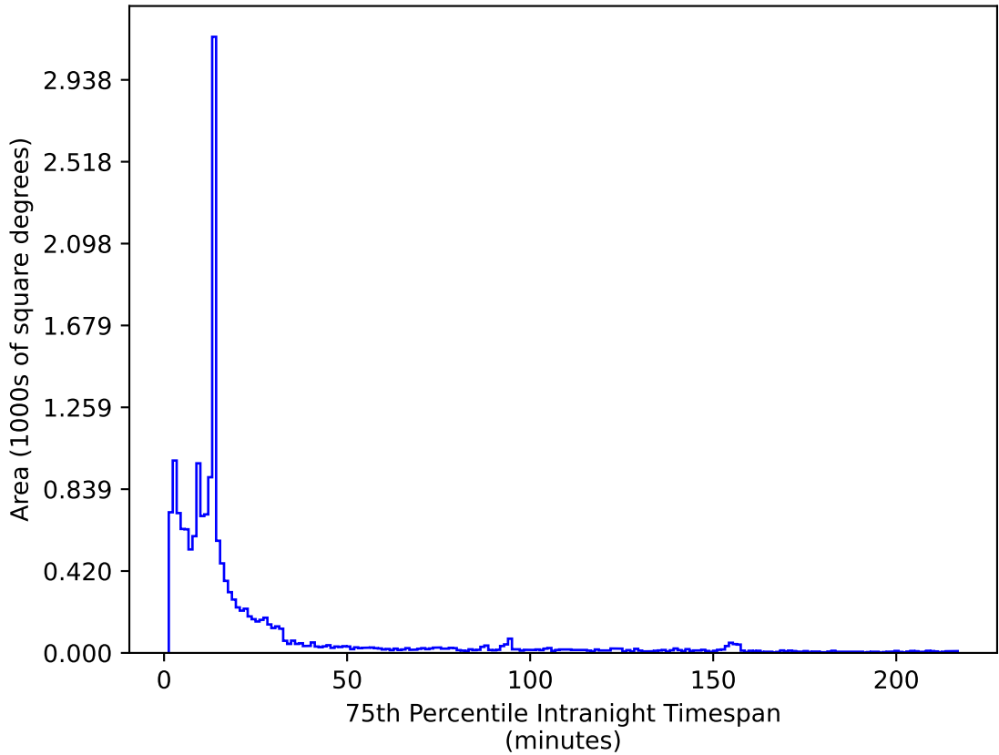
too_elab_r32_d3_griz_v3.4_10yrs WFD z band: 75th Percentile Intranight Timespan
