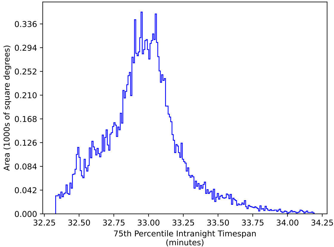
too_elab_r32_d3_griz_v3.4_10yrs WFD y band: 75th Percentile Intranight Timespan
