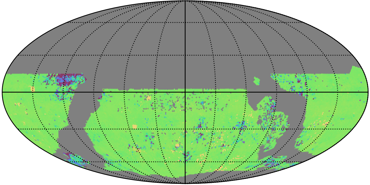
too_elab_r32_d3_griz_v3.4_10yrs WFD ug bands: 75th Percentile Intranight Timespan
