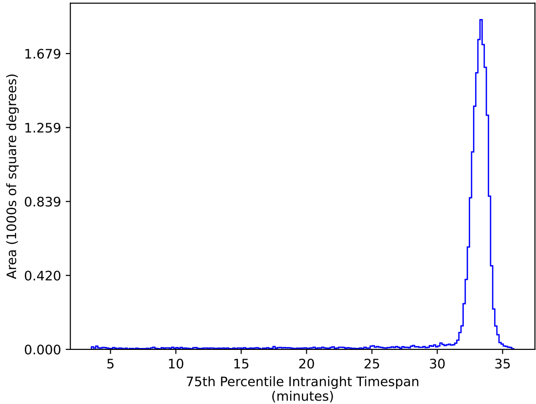
too_elab_r32_d3_griz_v3.4_10yrs WFD ug bands: 75th Percentile Intranight Timespan
