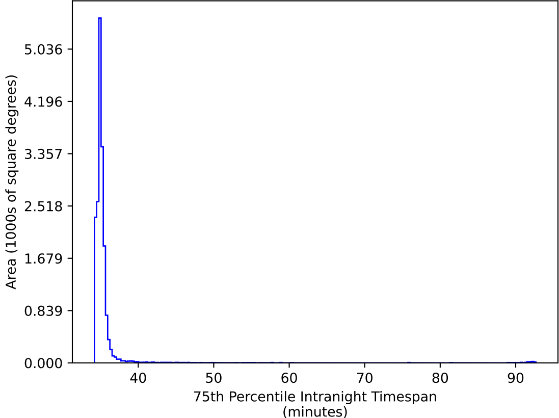
too_elab_r32_d3_griz_v3.4_10yrs WFD ri bands: 75th Percentile Intranight Timespan
