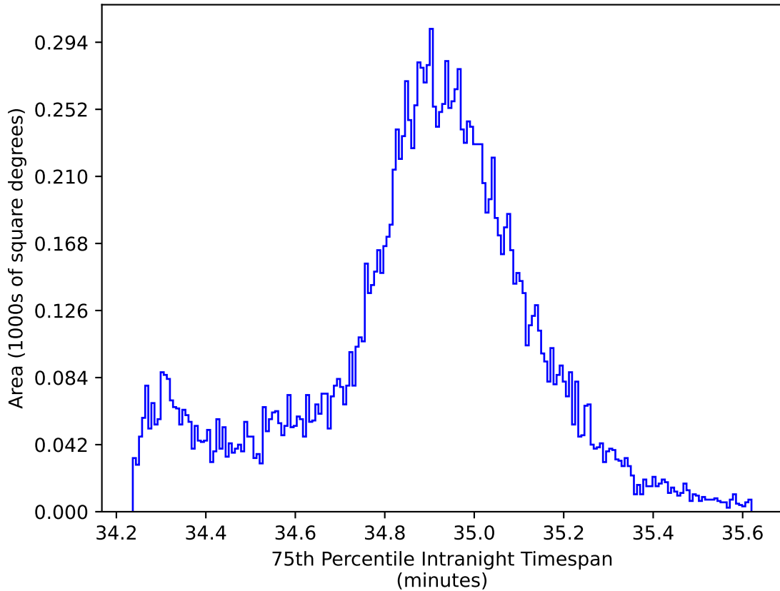
too_elab_r32_d3_griz_v3.4_10yrs WFD all bands: 75th Percentile Intranight Timespan
