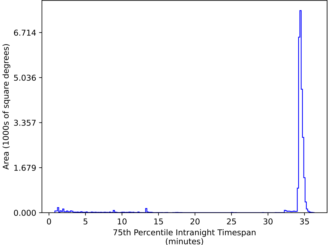
too_elab_r32_d3_griz_v3.4_10yrs All sky zy bands: 75th Percentile Intranight Timespan
