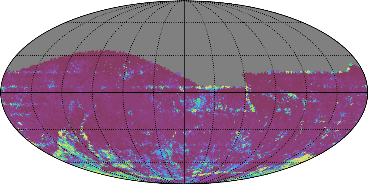
too_elab_r32_d3_griz_v3.4_10yrs All sky z band: 75th Percentile Intranight Timespan
