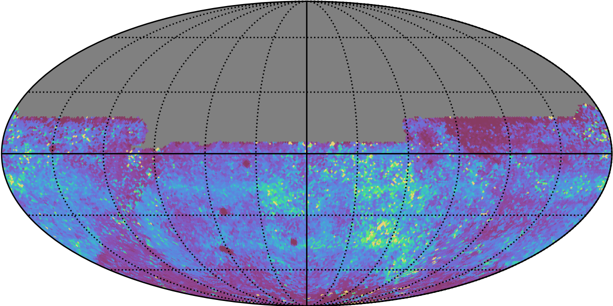
too_elab_r32_d3_griz_v3.4_10yrs All sky y band: 75th Percentile Intranight Timespan
